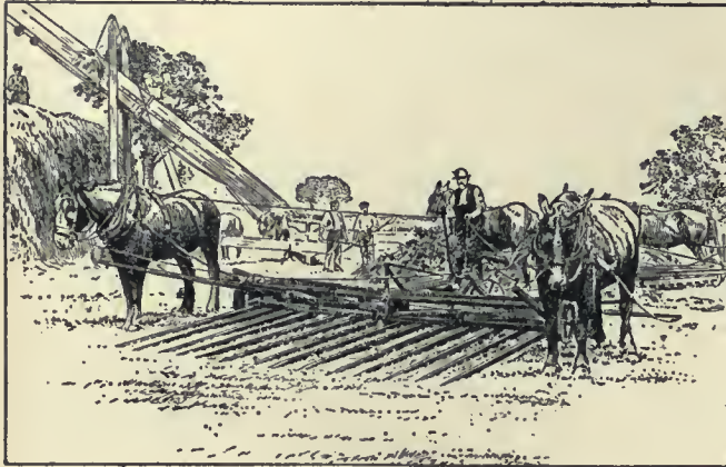
FIG. 5.—Sweep Rake.
